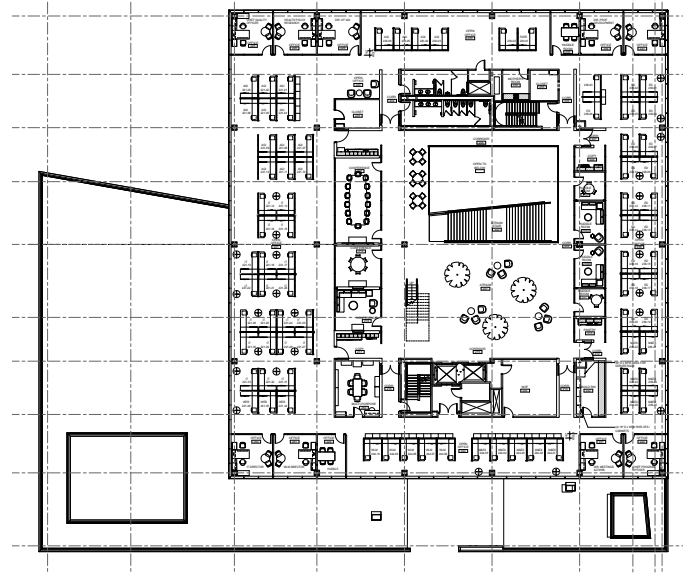
2ND FLOOR
